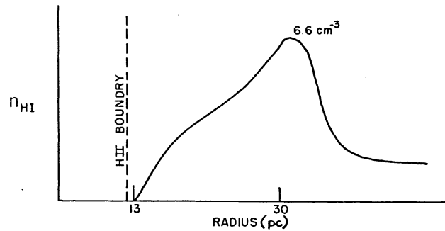
FIG. 2. Radial density distribution in the HI shell.
